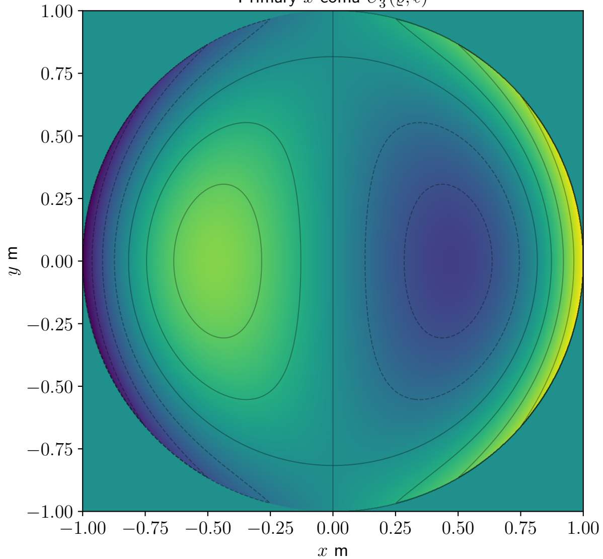
Primary x -coma U_3^1(\varrho, \ell)
