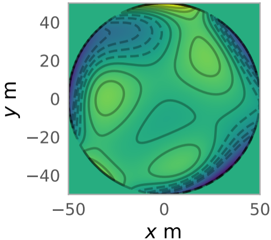
\varphi(x, y) no-tilt
